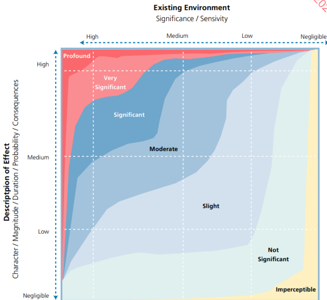
Figure 8.1: Determining Significance
